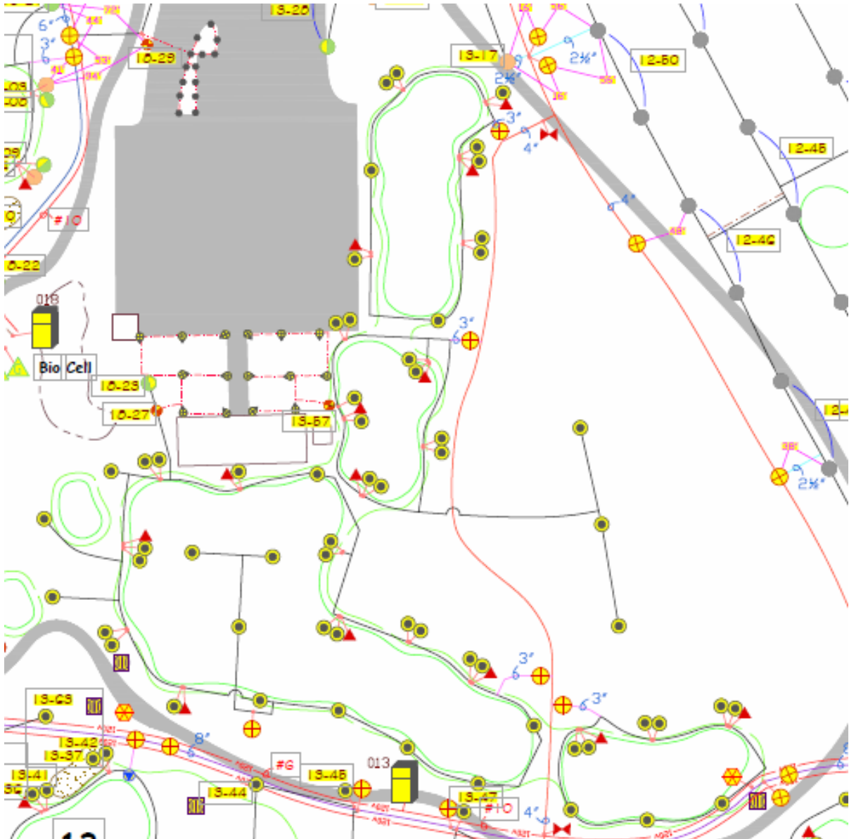
Figure 6. Proper irrigation systems improve water use efficiency. Putting course as-built at Palmer Hills 2021 Photo: Brian Hickey
